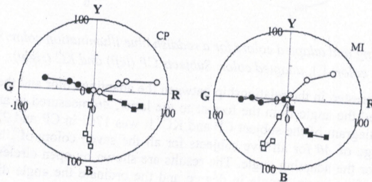
Fig. 6 Adapting and adapted colors for a red (open symbols) and green (filled) illumination. Circles, adapting color; Squares, adapted color. Subjects CP and MI.
