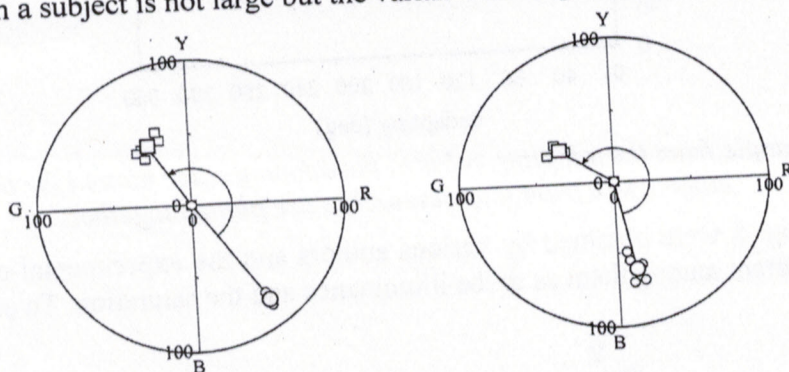
Fig. 4 Adapting and adapted colors for a reddish blue illumination color. \circ , adapting color; \square , adapted color. Subjects CP (left) and KC (right).
