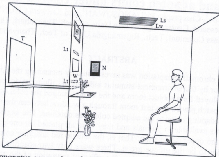
Fig. 1 Apparatus composing of a subject room (right) and a test room (left).
