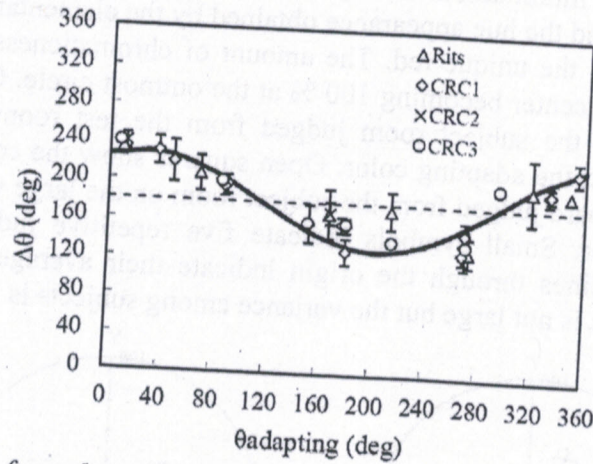
Fig. 5 The angle from the adapting color to the adapted color plotted for the adapting color. Data from four researches are plotted together.
