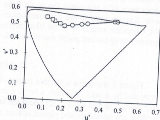
Fig. 3 Colors employed for the subject room illumination in the saturation experiment. \circ , red; \square , green.
