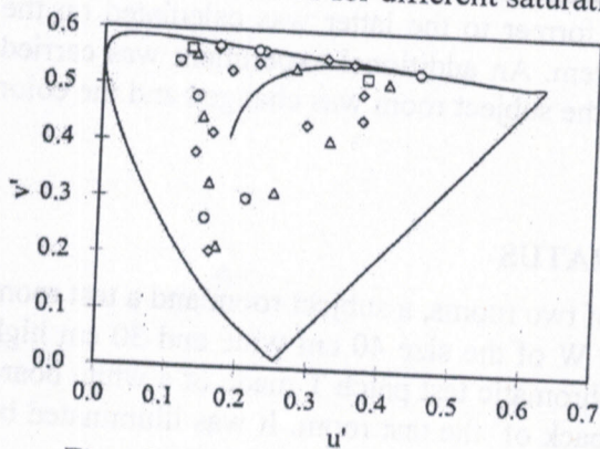
Fig. 2 Colors employed for the subject room illumination. \triangle , Rits 3) ; \diamond , CRC1 4) ; \square , CRC2 2) ; \circ , CRC3, present work.
